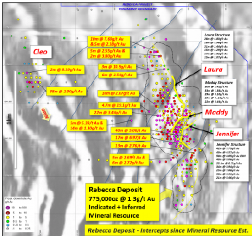
Apollo Consolidated Limited Lake Rebecca drill plan
